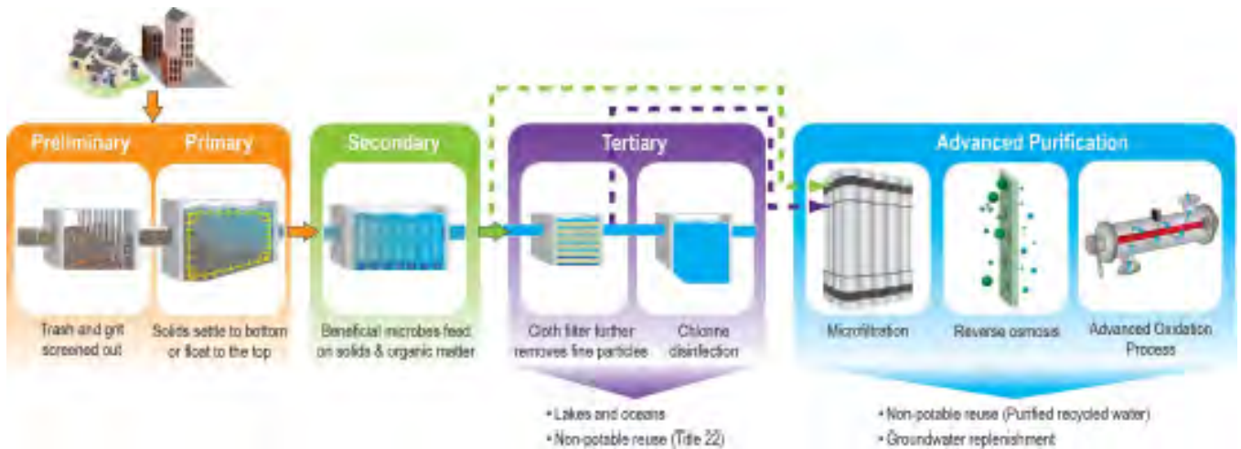
General Recycled Water Process Diagram 2
